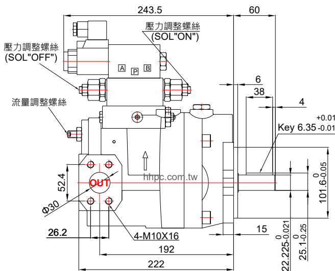
P36/46-E*-F-R-TYPE
