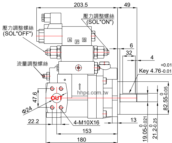
P36/46-E*-F-R-TYPE
