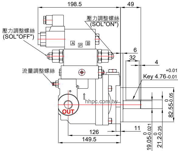
P08/10/13-E*-F-R-TYPE
