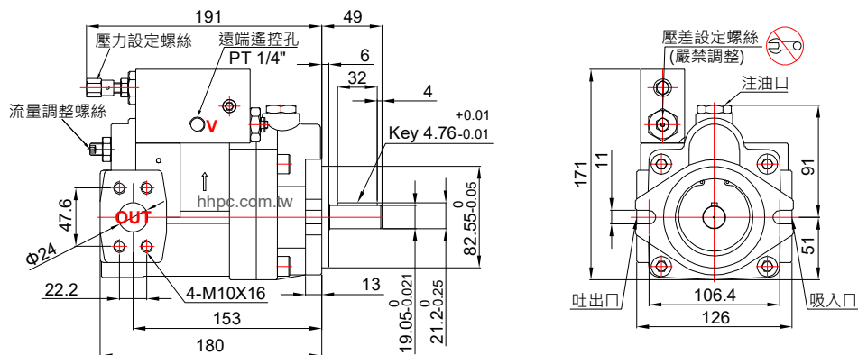
P16/22-BH*-F-R-TYPE
