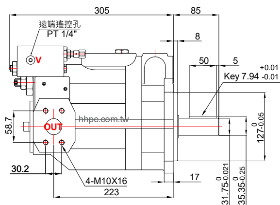
P100-A*-F-R-TYPE
