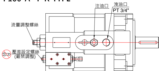
P100-A*-F-R-TYPE
